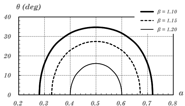
Fig. 3 The dependence of the stable inclined attitude \theta on material \alpha .
