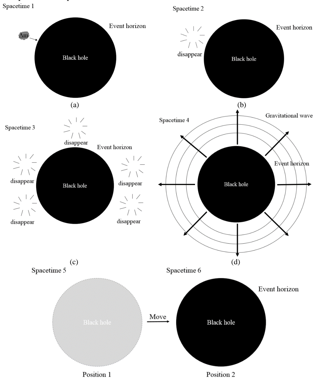
Figure 1. (a) The Spacetime 1 before something enters into the black hole. (b) The Spacetime 2 after 3
