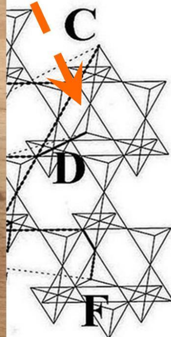
Figure 9, A stable black hole nucleus is large enough to “eat” the vacuum particles and grow by it.
