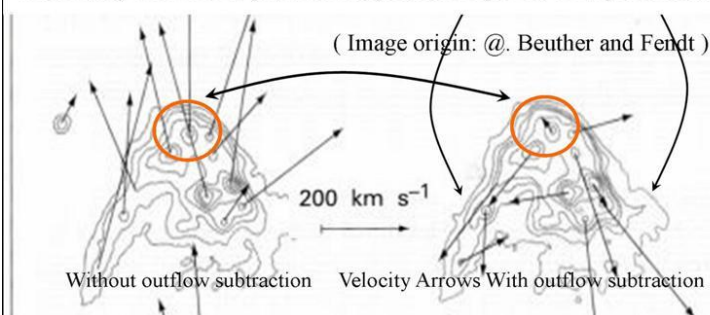
Figure 35. Example of NGC 326: The Repelling of Two Equal sized Black Holes as the formation of a Herbig Haro Bowshock system, with star formation in between and double jets. According to Quantum FFF Theory.
