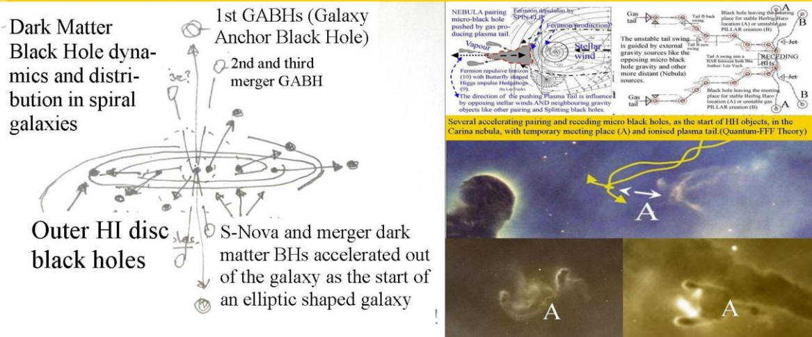
Figure, 29 . Dark Matter Black Hole dynamics in spiral galaxies.
