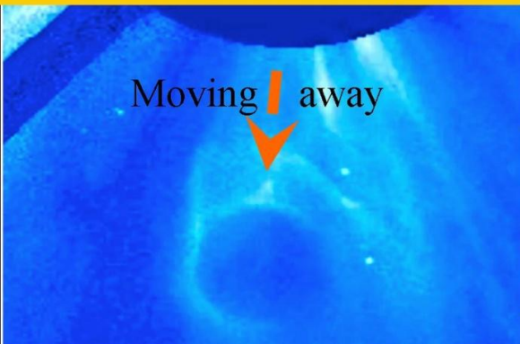
Figure 23, Even the sun seems to have polar dual black hole Herbig Haro remnants and is able to produce and expel gas planets (failed stars) at this age.
