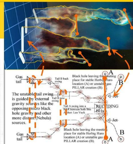
Figure 35. Example of NGC 326: The Repelling of Two Equal sized Black Holes as the formation of a Herbig Haro Bowshock system, with star formation in between and double jets. According to Quantum FFF Theory.
