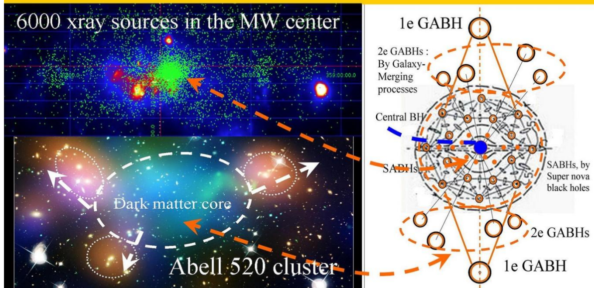
Figure 5, Merger dynamics of NON inertial Dark Matter black holes left behind after merging in the middle.
