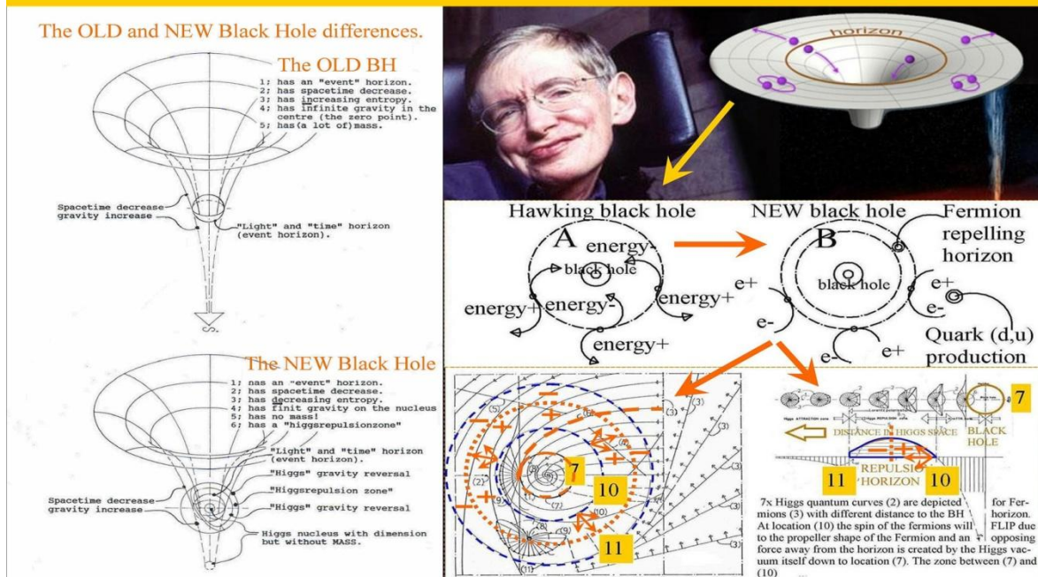
Figure 30, The new black hole
