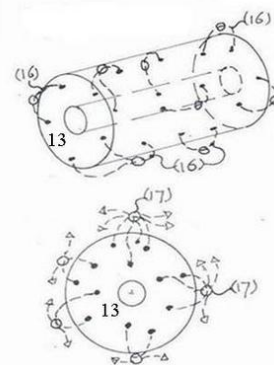
Figure 16, BBBH , the Big Bang Black Hole splintering into smaller BHs and evaporating into the oscillating Axion Higgs Vacuum lattice .
