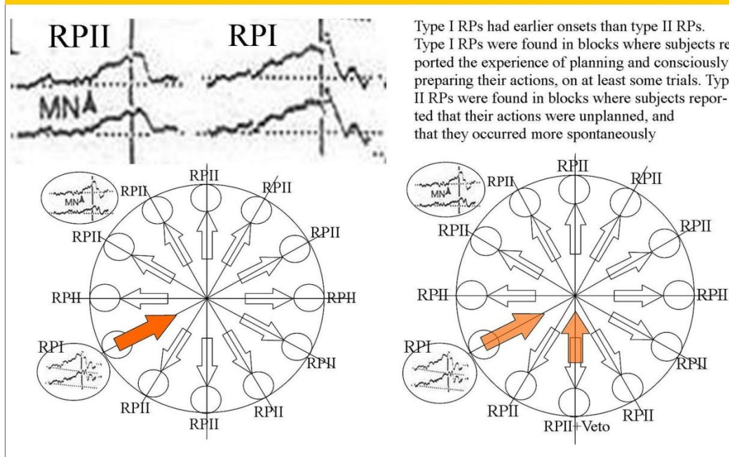
Figure 32, Quantum FFF Theory explanation of the difference between RPI and RPII ( R=Readiness potential) observed and published by Benjamin Libet around 1964. ( reference: 72: Democratic Free Will and Telepathy in the Instant Entangled Multiverse )
