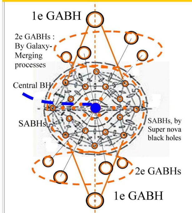
Figure 15, GABHs as the largest unit of Dark Matter black hole families
