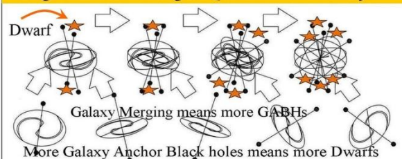
Figure 15, GABHs as the largest unit of Dark Matter black hole families
