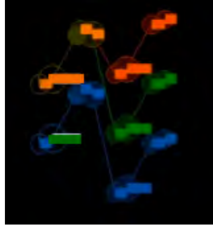
D4 Standard Model
