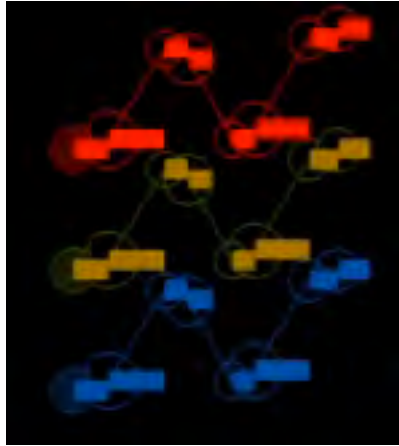
D4 Gravity+Dark Energy
