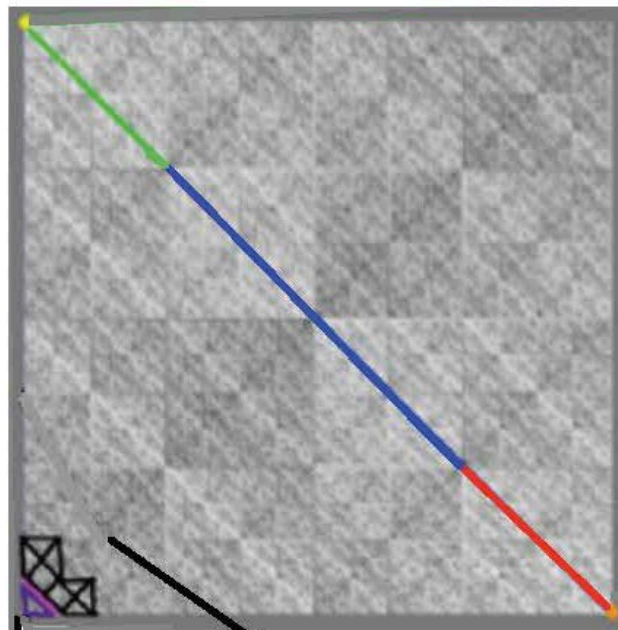
Cl(16) 256x256 Matrix Representation
