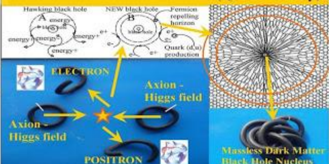
Figure 22, The extended Standard Model according to Quantum FFF Theory, ( Function Follows Form, at the quantum scale and above)
