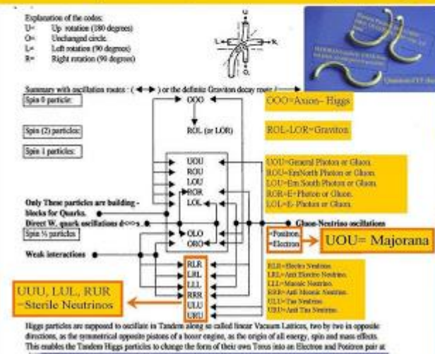
Figure 22, The extended Standard Model according to Quantum FFF Theory, ( Function Follows Form, at the quantum scale and above)
