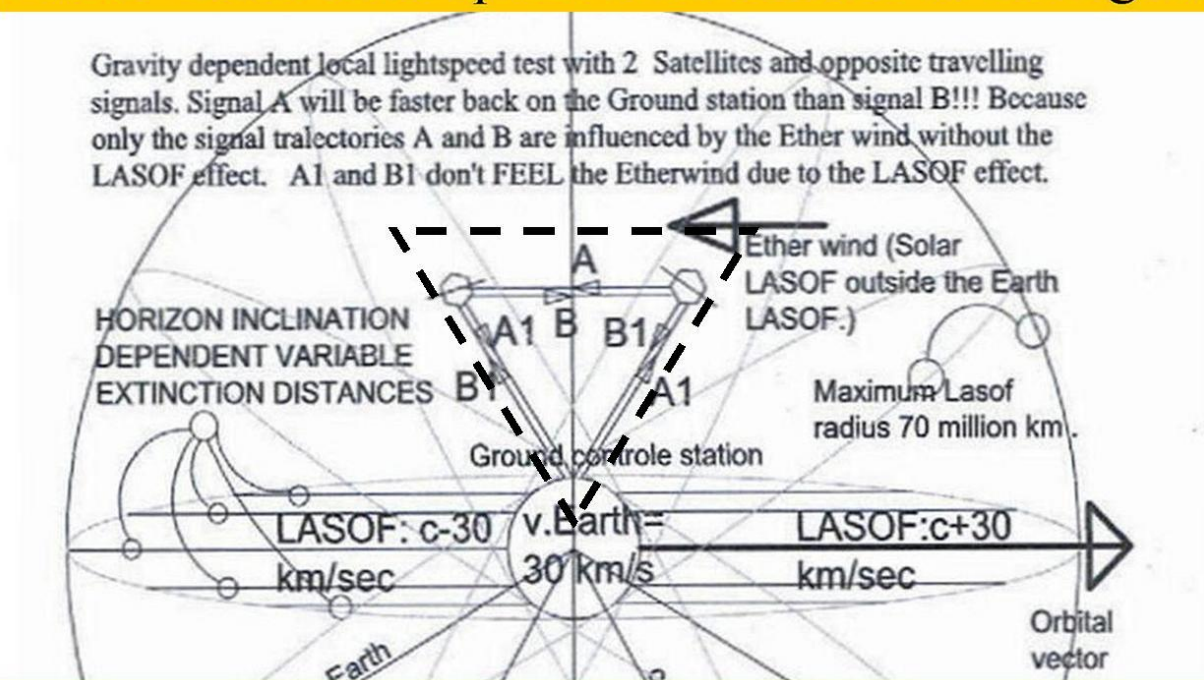
Figure 10. Michelson Morley experiment revised.
