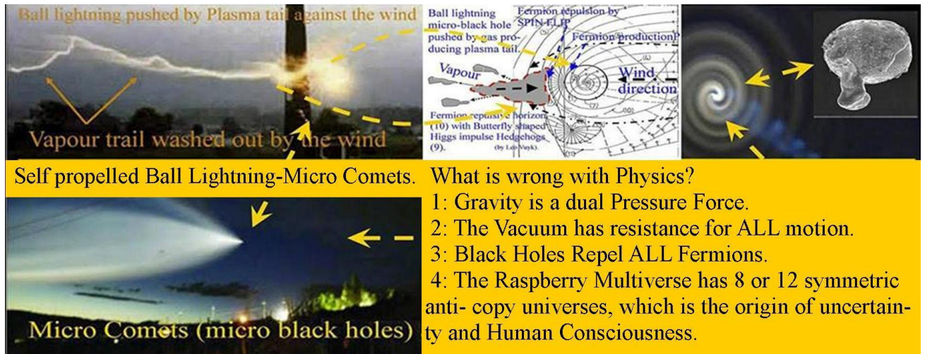
Figure 1, Waht is wrong with physics on earth and in space.
