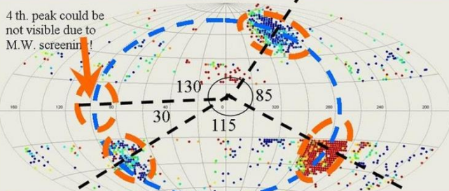
Figure 5. The cube- and cube octahedron multiverse configuration, based on three or four fluctuation anomalies.
