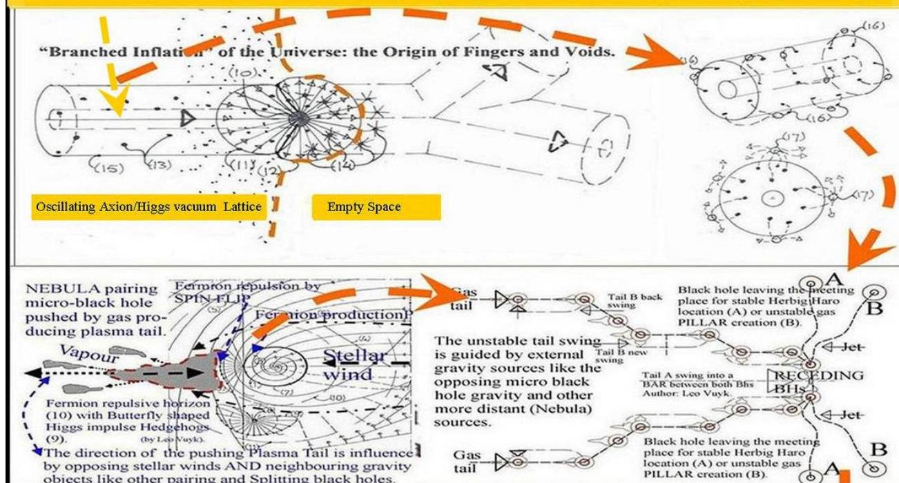
Figure 6, The bouncing multiverse poster.
