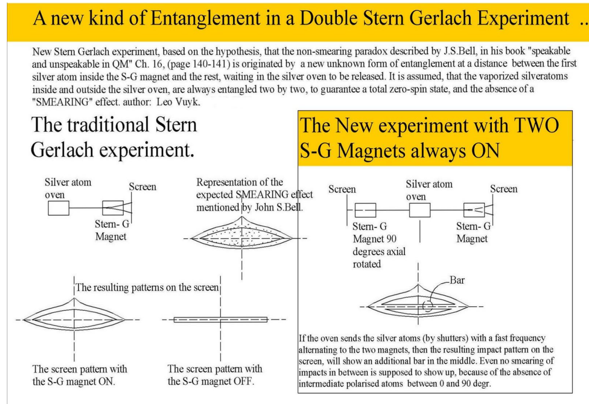
Figure 8, To solve the Q.M. problem described by J.S.Bell about the standard Stern Gerlach experiment. Experiment proposal to support the existence of a new kind of Entanglement, which should show up inside a double Stern Gerlach experiment with two S-G magnets with different orientation.
