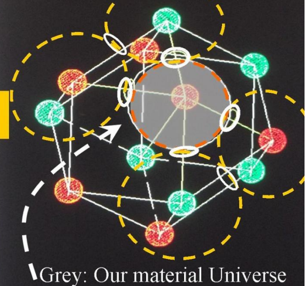
Figure 5. The cube- and cube octahedron multiverse configuration, based on three or four fluctuation anomalies.
