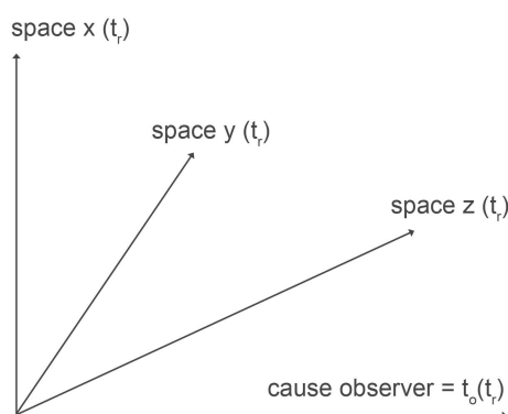
Figure 5. : creating 4-dimensional spacetime
