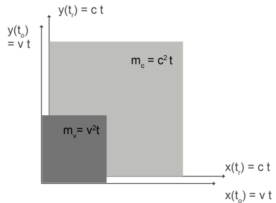
Figure 6. : creating 4-dim. spacetime with 2x2 dimensional space
