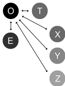
Figure 3. : Observer creating (empty) 4-dim. space-time by finding 6 elementary particles.
