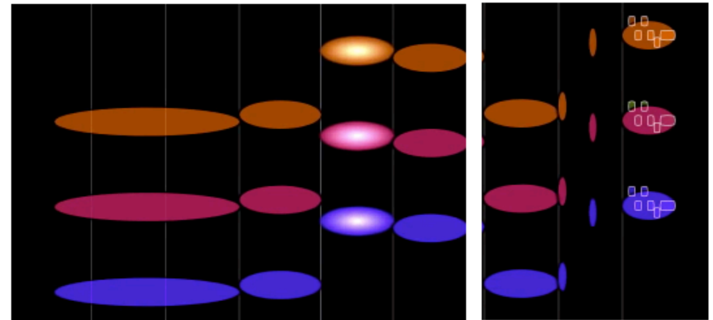
M4 M4 x CP2 Kaluza-Klein Quaternionic Spacetime CP2 = SU(3)/U(2)
