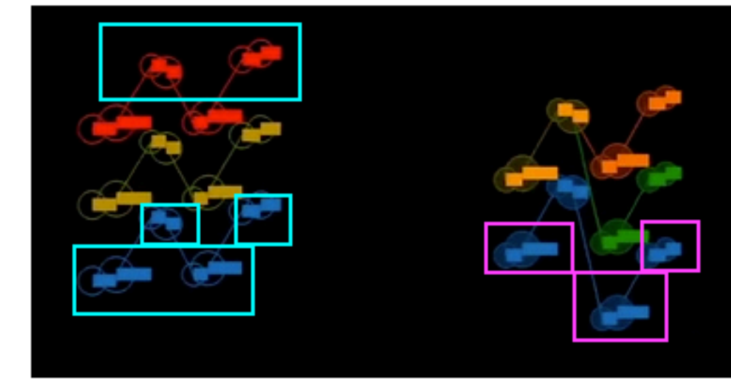
8 Standard Model Root Vectors
