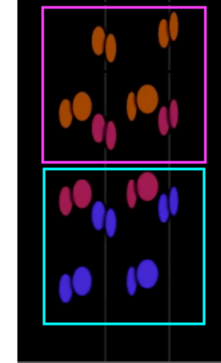
12 SU(2,2) Root Vectors
