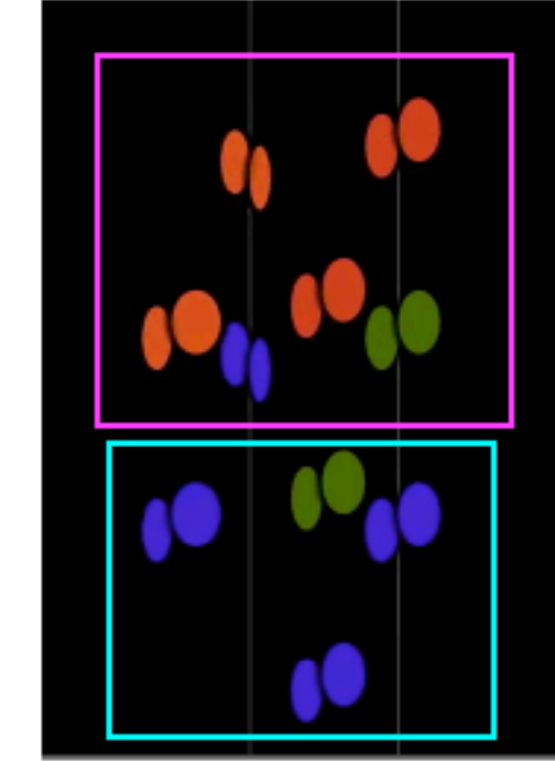
8 Standard Model Root Vectors
