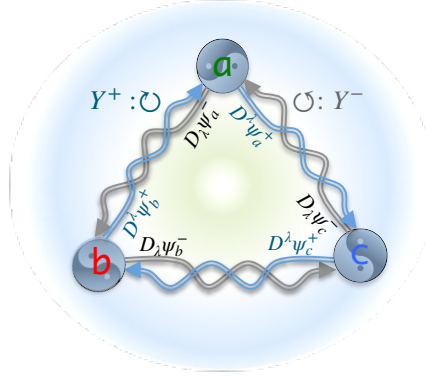
Figure 2.0b: Ontological Evolutions
