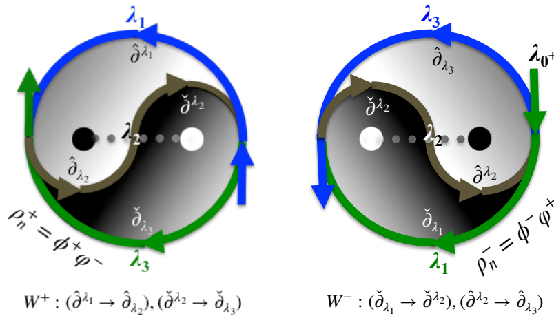
Figure 2.0a: Events of YinYang Processes : \hat{\partial}^\lambda \cup \hat{\partial}_\lambda = \check{\partial}^\lambda \cup \check{\partial}_\lambda
