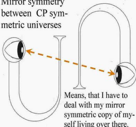
Figure 4, wavefunction collapse between CP symmetric mirror particles by instant entanglement between multi universal bubbles located around the Big Bang central void.
