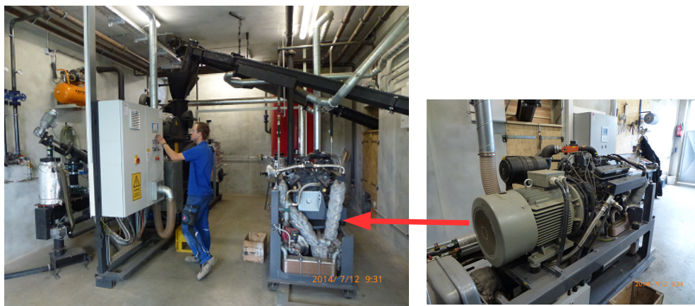
Fig. 5. Spanner Re 2 wood gas cogenerator installed by Josef Strobl Heizung Solar in Giglberg and Velden/Vils/Lower Bavaria/Germany. Left: pyrolysis unit in left image half. Gas engine and generator on right half. Right: enlarged image of Gas engine and generator.
