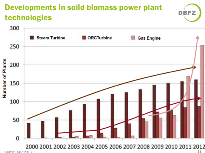
Fig 6. Development of solid biomass power plant technologies. Pink bars and trend curve for gas engines, i.e. predominantly wood gasification [Lenz 2014].
