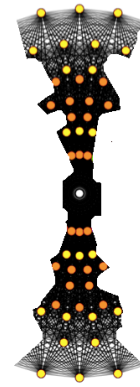
E_8 8D gauge bosons + ghosts
