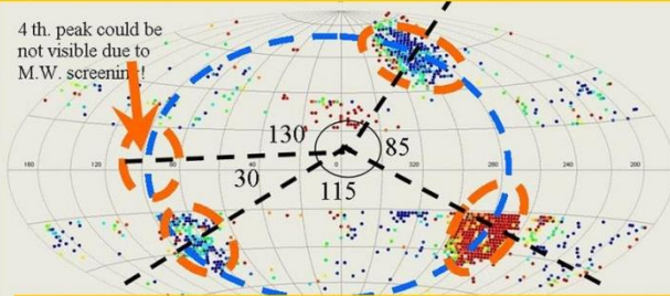
Figure 15, Our position in a 8 or even 12 fold multiverse based on fluctuation anomalies (universal contact areas)
