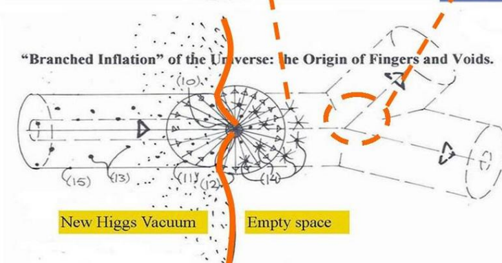
Figure 10 , BBBH , the Big Bang Black Hole splintering into smaller BHs and evaporating into the oscillating Axion Higgs Vacuum lattice .
