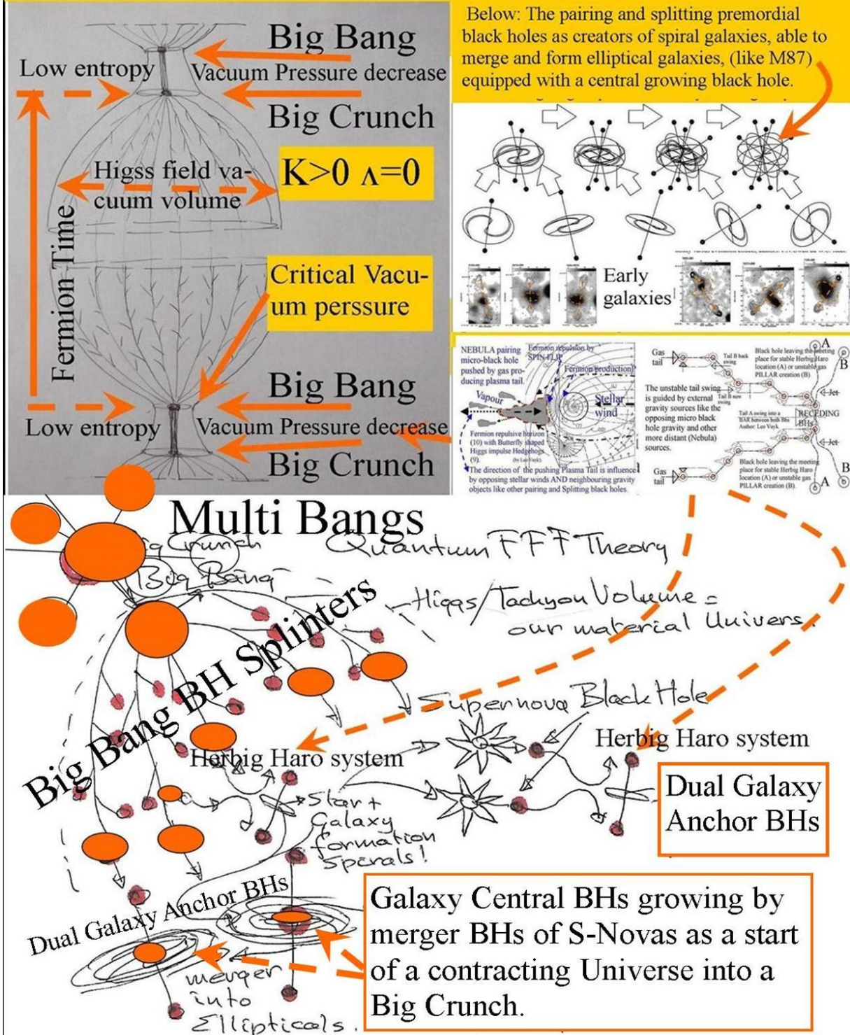
Figure 13, The Cyclic Multiverse.
