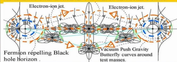
Figure 17, Even the sun seems to have polar dual black hole Herbig Haro remnants and is able to produce and expel gas planets (failed stars) at this age.
