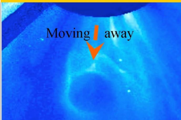
Figure 17, Even the sun seems to have polar dual black hole Herbig Haro remnants and is able to produce and expel gas planets (failed stars) at this age.
