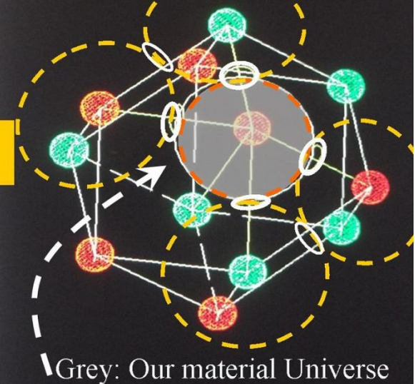
Figure 15, Our position in a 8 or even 12 fold multiverse based on fluctuation anomalies (universal contact areas)
