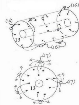
Figure 10 , BBBH , the Big Bang Black Hole splintering into smaller BHs and evaporating into the oscillating Axion Higgs Vacuum lattice .
