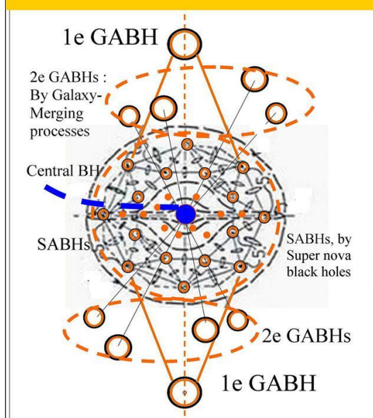
Figure 1. Simple external (new physics) black hole configuration.
