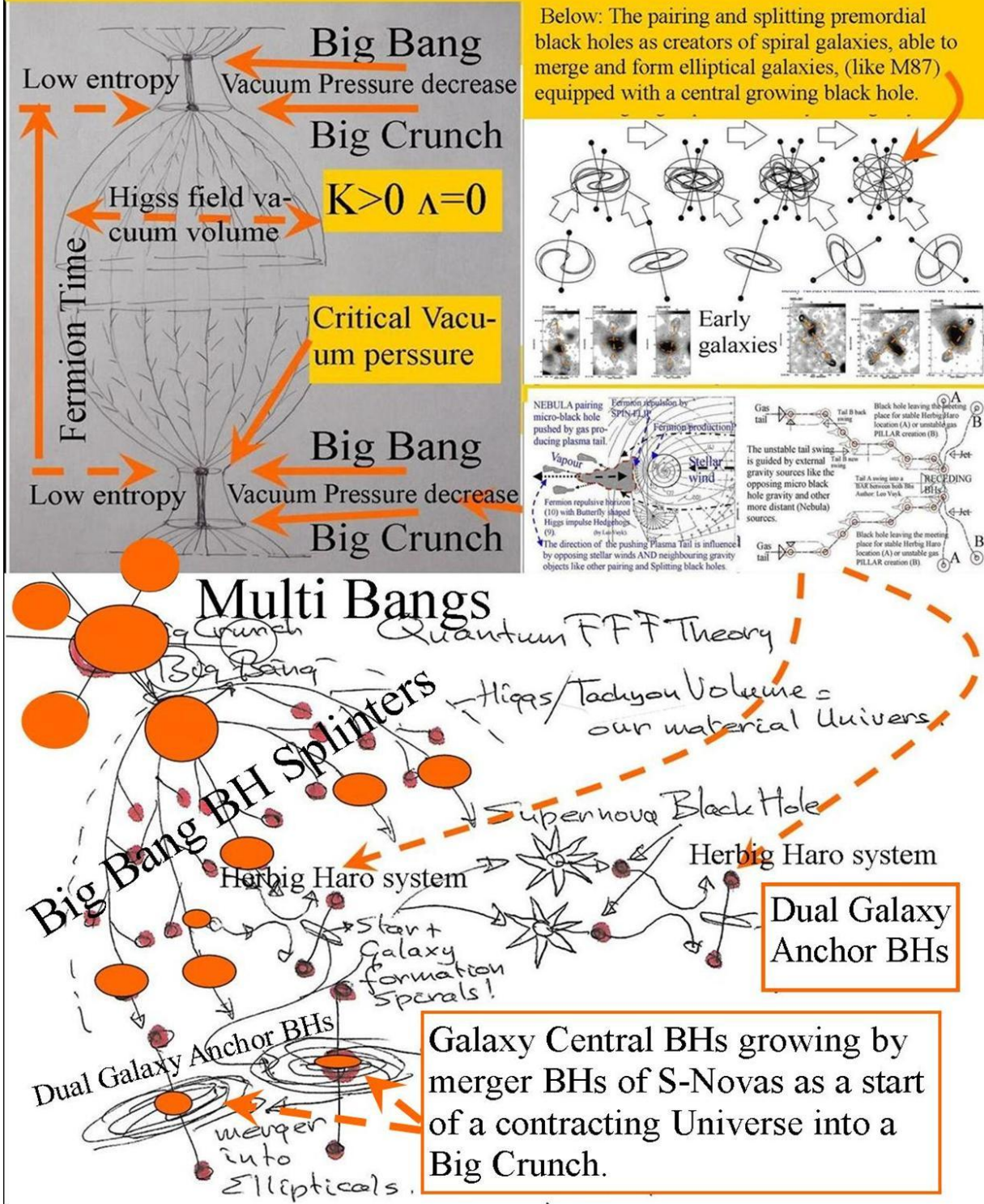
Figure 3. Big Bang black hole splinters as the creators of pairing BH Herbig Haro systems according to Q-FFF Theory.
