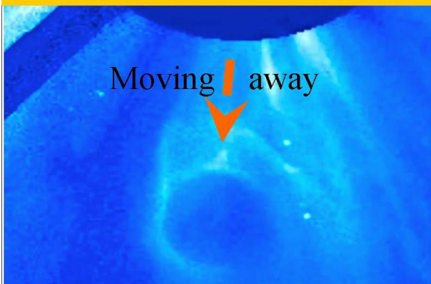
Figure 6, Even the sun seems to have polar dual black hole Herbig Haro remnants.
