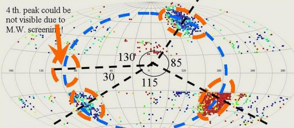
Figure 7. 8 or 12 fold raspberry multiverse proposal.
