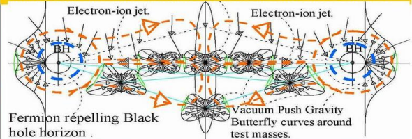
Figure 6, Even the sun seems to have polar dual black hole Herbig Haro remnants.
