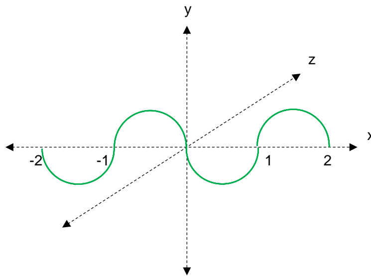
Figure 8; for the trace value of \frac{-1}{\varphi} we would reach a value of \pi in each direction of the x-axis (here as the value of “2” in each direction of the x-axis, the overall trace length for this sinusoidal wave would represent a value of 2\pi in factoring in the dual directions along the x-axis from the 0 reference, \pi along each direction symbolised as “2” semicircular diametres.
