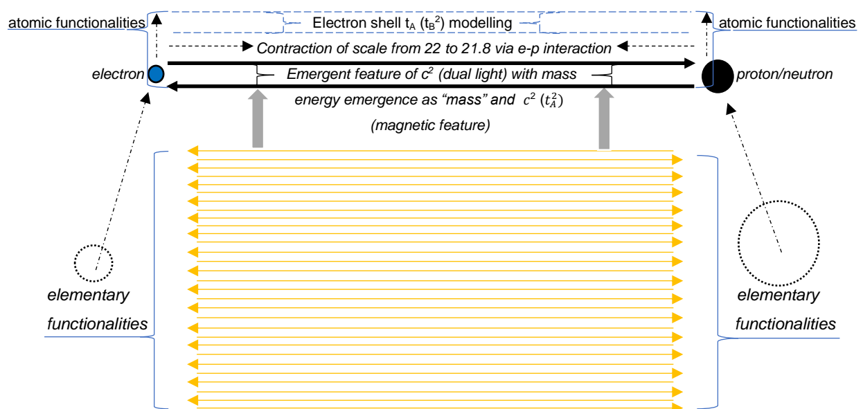
Figure 16; “beyond” the 30c manifold is a “ c ” factor that can only be “squared” as a “future” ( t_A^2 ) event beyond the primary 30c “now” event. Note also the contraction of the atomic scale from 22 to 21.8 owing to the emergent force between the electron and the proton, and subsequent electron shell modelling.
