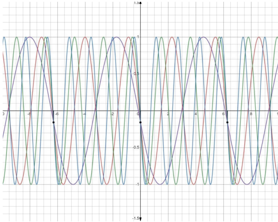
Figure 5 Sampling and Harmonics
