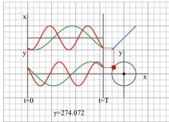
Figure 20 The Effect of a Phase Shift
