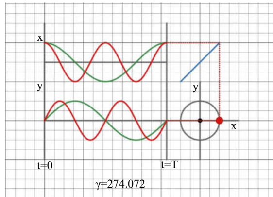
Figure 18 The Second Energy State
