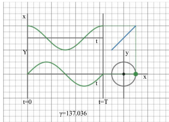
Figure 16 The Base Energy State
