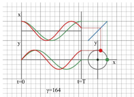
Figure 17 An Unstable State
