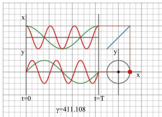
Figure 19 The Third Energy State
