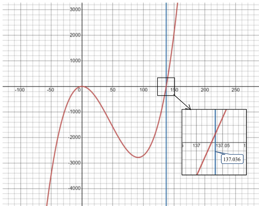
Figure 21 Graph of Cubic
