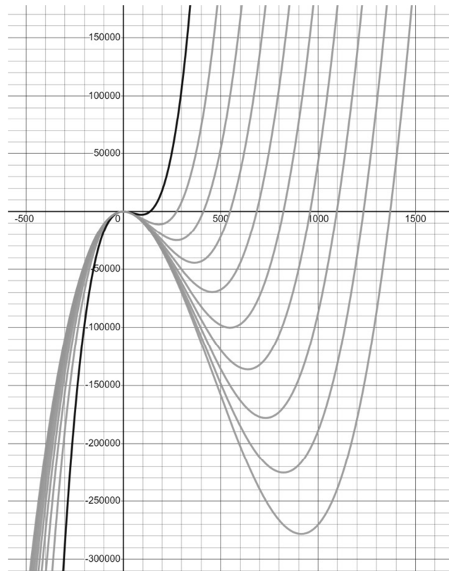
Figure 22 Graph of y = \frac{\alpha}{n} \gamma^3 - \gamma^2 + 1
