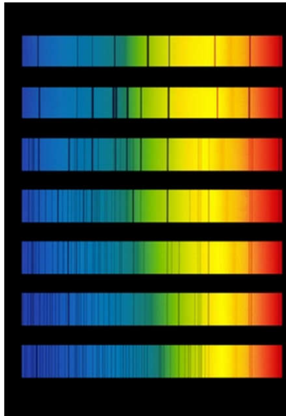
Figure 1 Absorption Spectra
