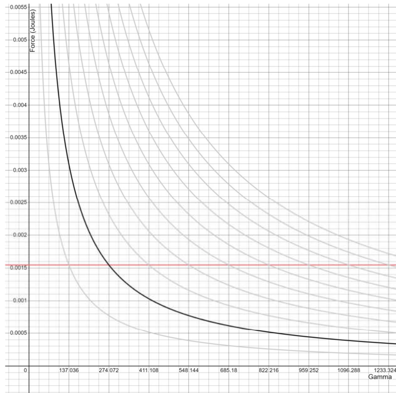
Figure 23 Family of Curves of Force vs Gamma
