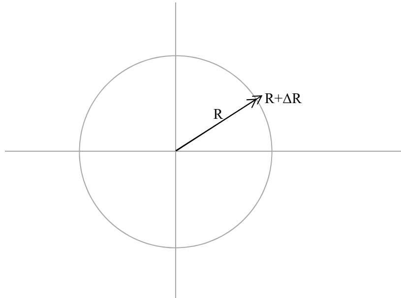
Figure 24 A small change in orbital radius
