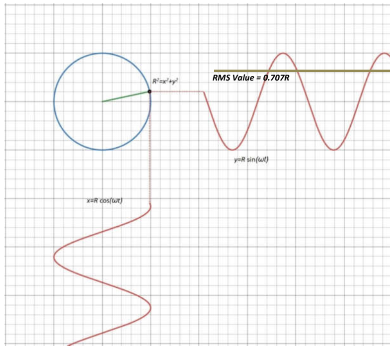
Figure 26 Parametric equations for the orbiting electron
