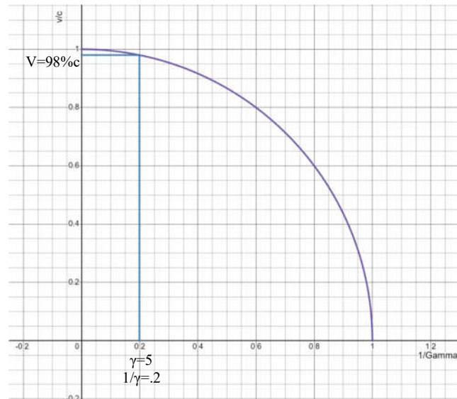
Figure 10 Reciprocal of Gamma
