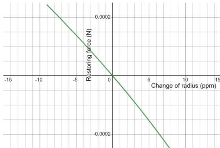
Figure 25 Restoring force vs Change of Radius
