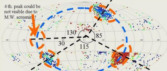
Figure 2, Our position in the 8 or 12 fold multiverse.
