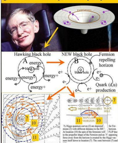
Figure18, Universal cyclic dynamics
