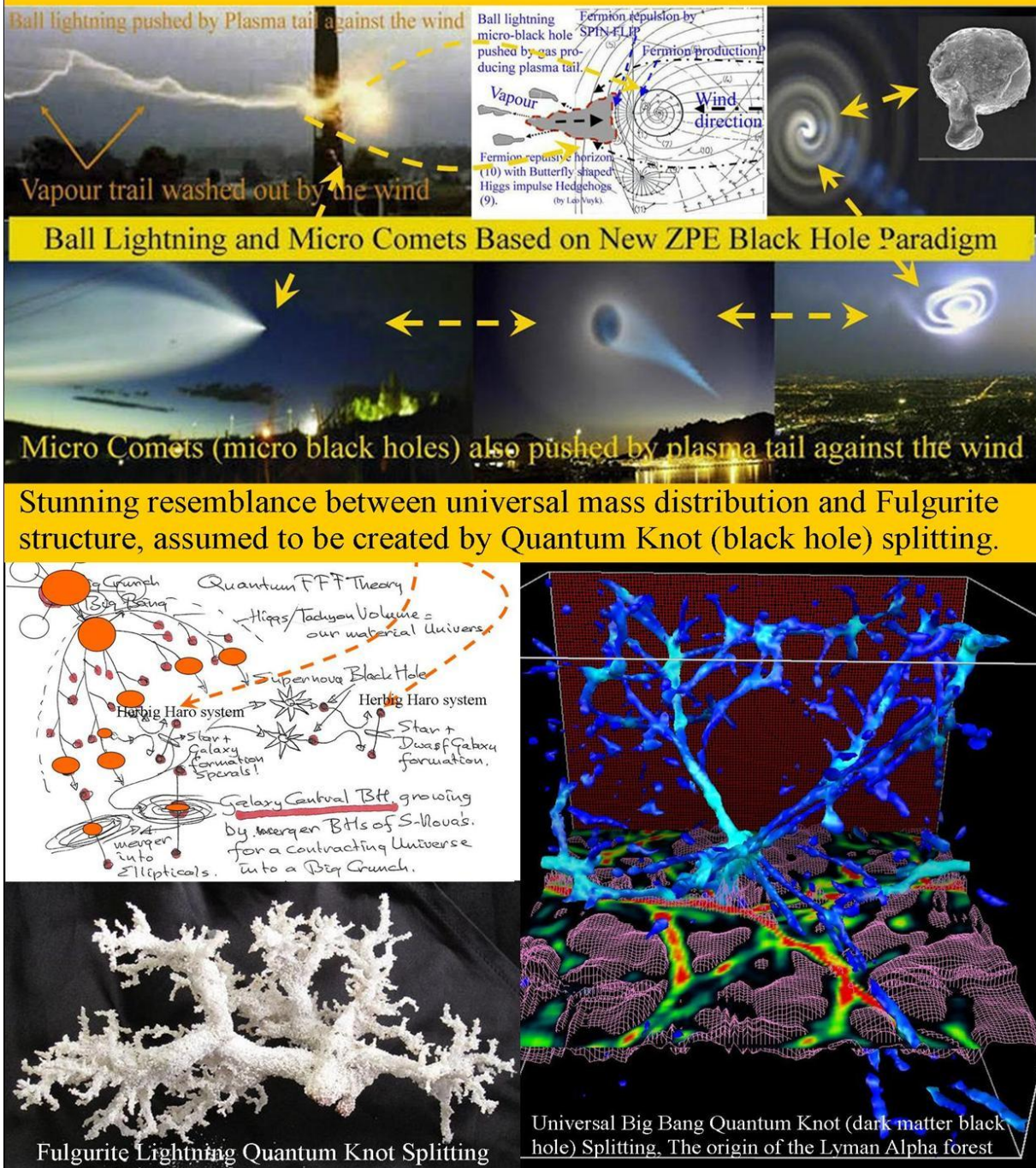
Figure 17, Black holes can have all sizes, from ball lightning up to the Big Crunch black hole.
