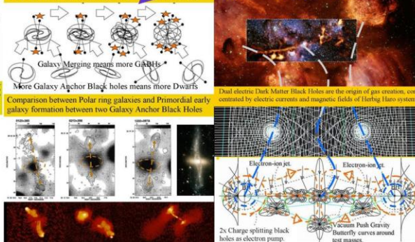
Figure 16, star formation and dying according to Quantum-FFF Theory.
