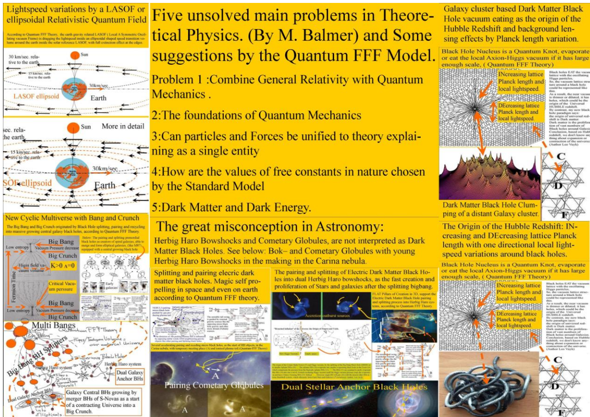
Figure: 13, Five unsolved problems in Physics.
