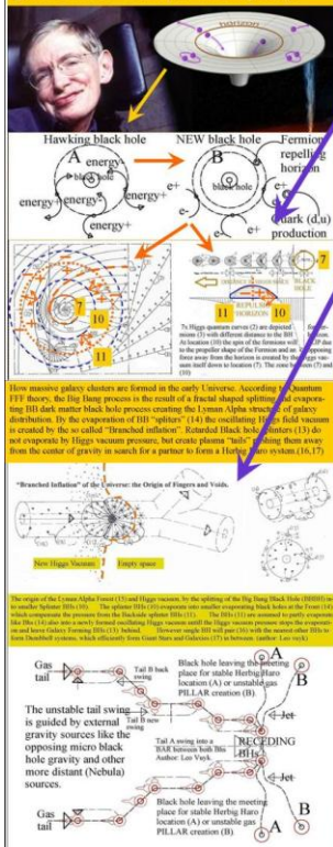
Figure 16, star formation and dying according to Quantum-FFF Theory.
