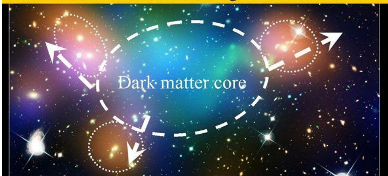
Figure: 14, Dark Matter Black Hole Peakes in dark matter core of a Galaxy cluster.
