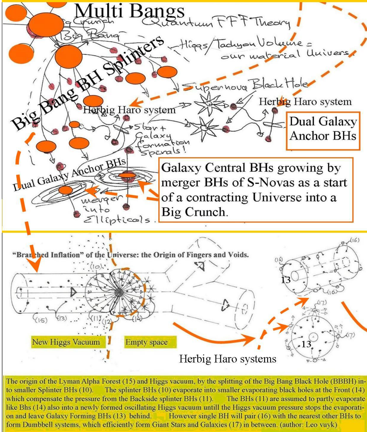
Figure 9, The cyclic multiverse with BigCrunch and Big Bang.
