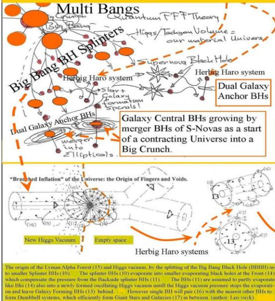
Figure: 10, B Bang Black Hole Nucleus Splitting and Pairing Process after a Big Crunch of the Raspberry Multiverse .
