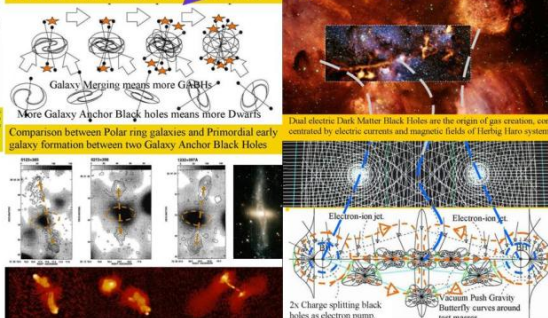
Figure 5, The new paradigm of star/galaxy formation and dying.
