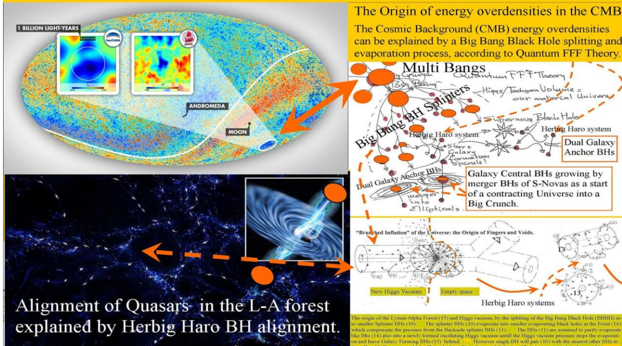
Figure: 12, Cold Spot alignment with the Supervoid. As location for the BigBang.
