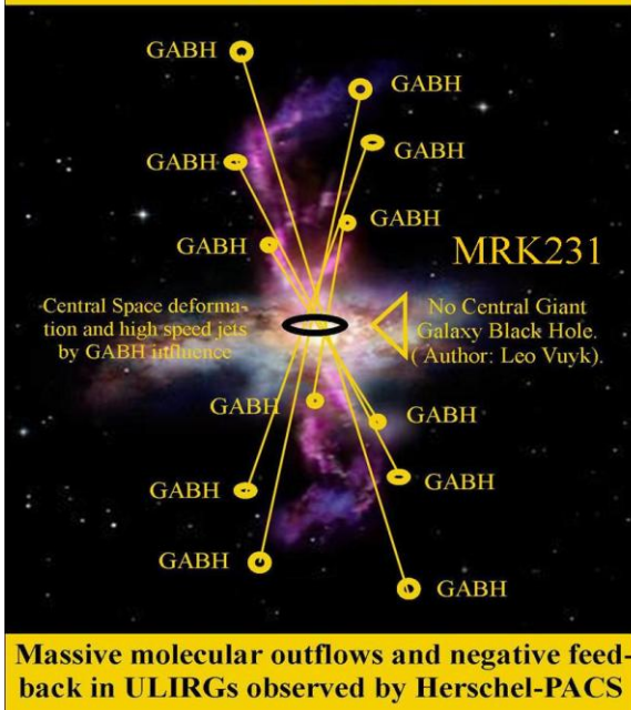
Figure 15, Primordial Galaxy Anchor black holes.
