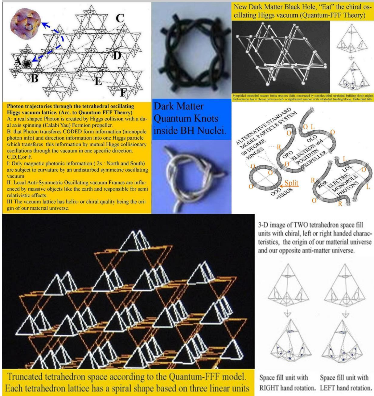
Figure 8, the superconducting vacuum lattice.
