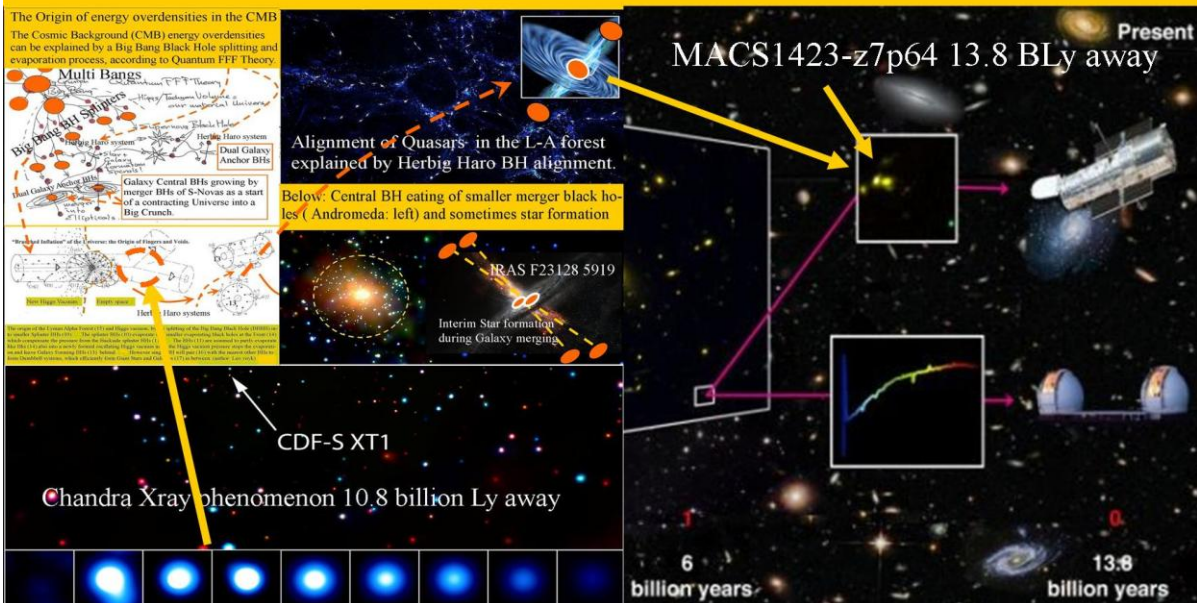
Figure: 11, Single and Double Black Hole signals in the early universe.
