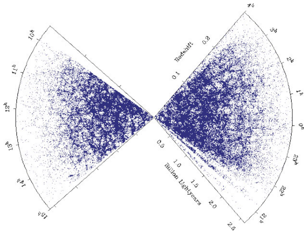
Figure 1. 2dF SDSS Galaxy Redshift Survey [27] .
