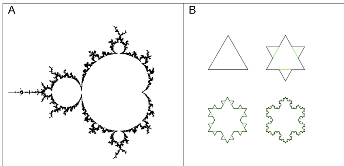
Figure 3. (Classical) Fractals: (A) boundary of the Mandelbrot set; (B) The Koch Snowflake fractal from iteration 0 to 3. Reference: (A) [31]; (B) [32].
