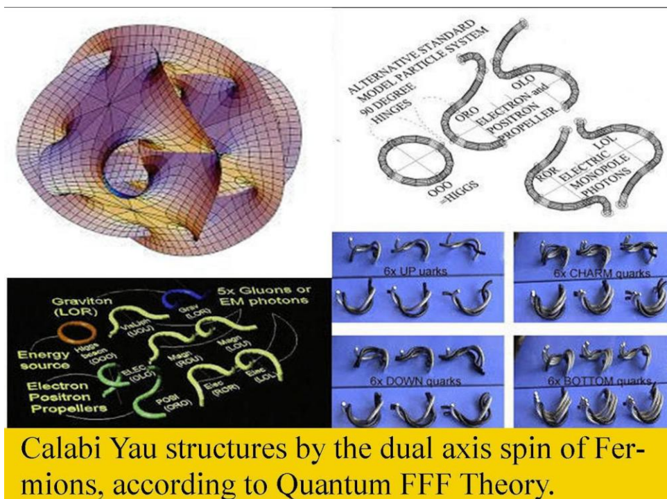
Figure 1 Several sub quantum shaped particles suggested by Quantum FFF Theory
