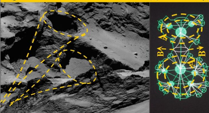
Figure 11, Gravity anomalies by aligned earth internal dark matter black holes.
