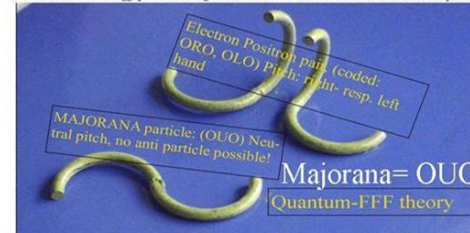
Figure 4, particle schemes of Quantum FFF Theory.
