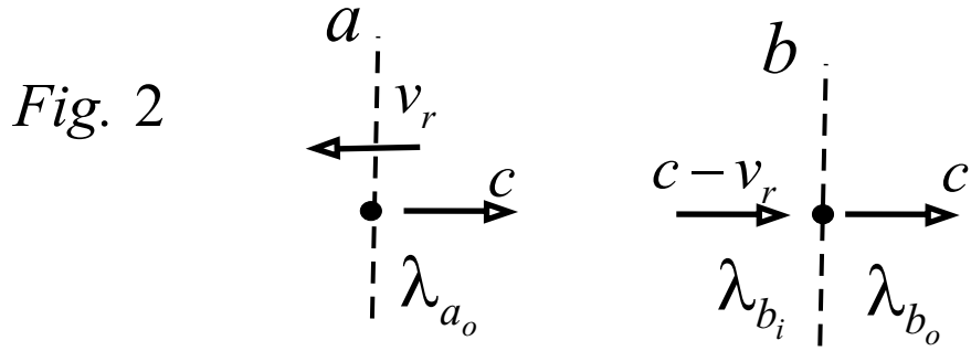
Figure 32: Sagnac experiment
