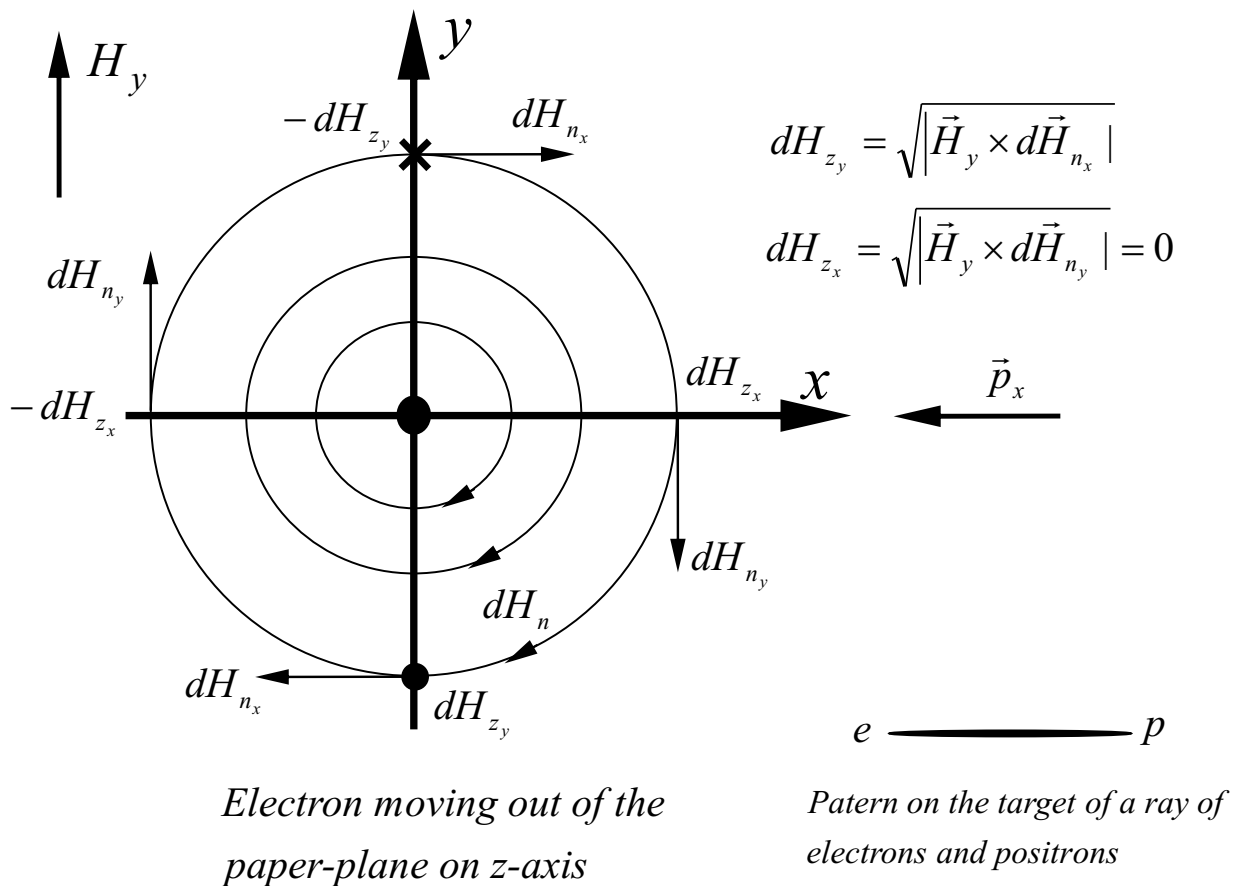
Figure 10: Stern-Gerlach-experiment with an homogeneous magnetic field
