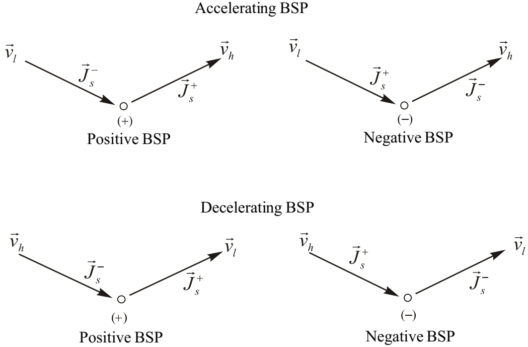
Figure 21: Conventions for BSPs
