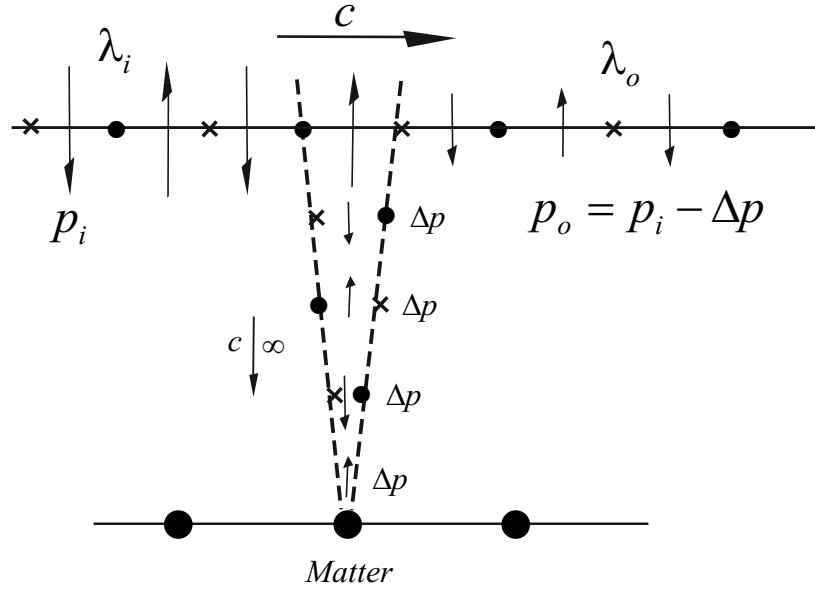
Figure 33: Loss of energy of a BSP with v = c
