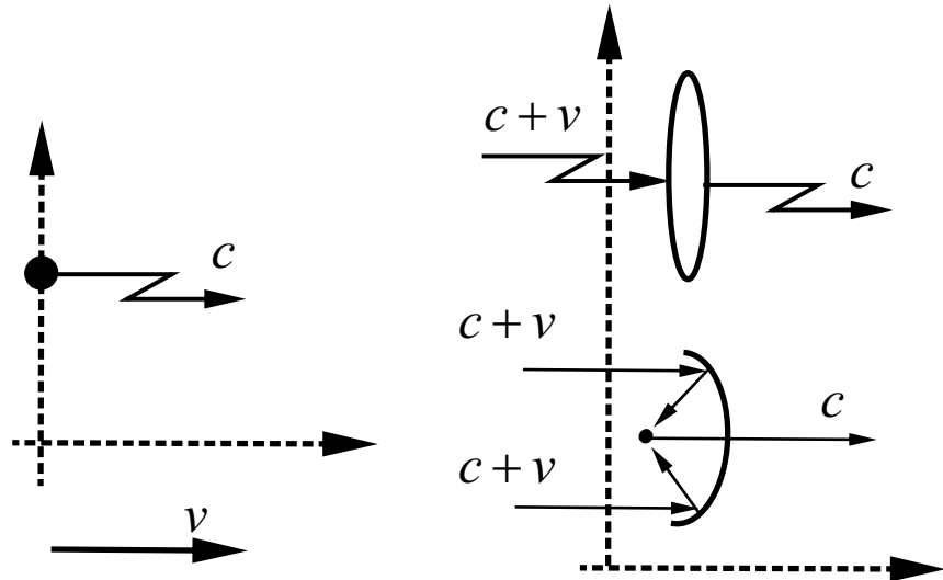
Figure 28: Light on relative moving receivers
