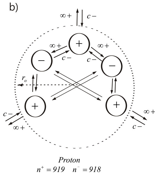
Figure 22: Neutron and proton composed of accelerating positrons and decelerating electrons
