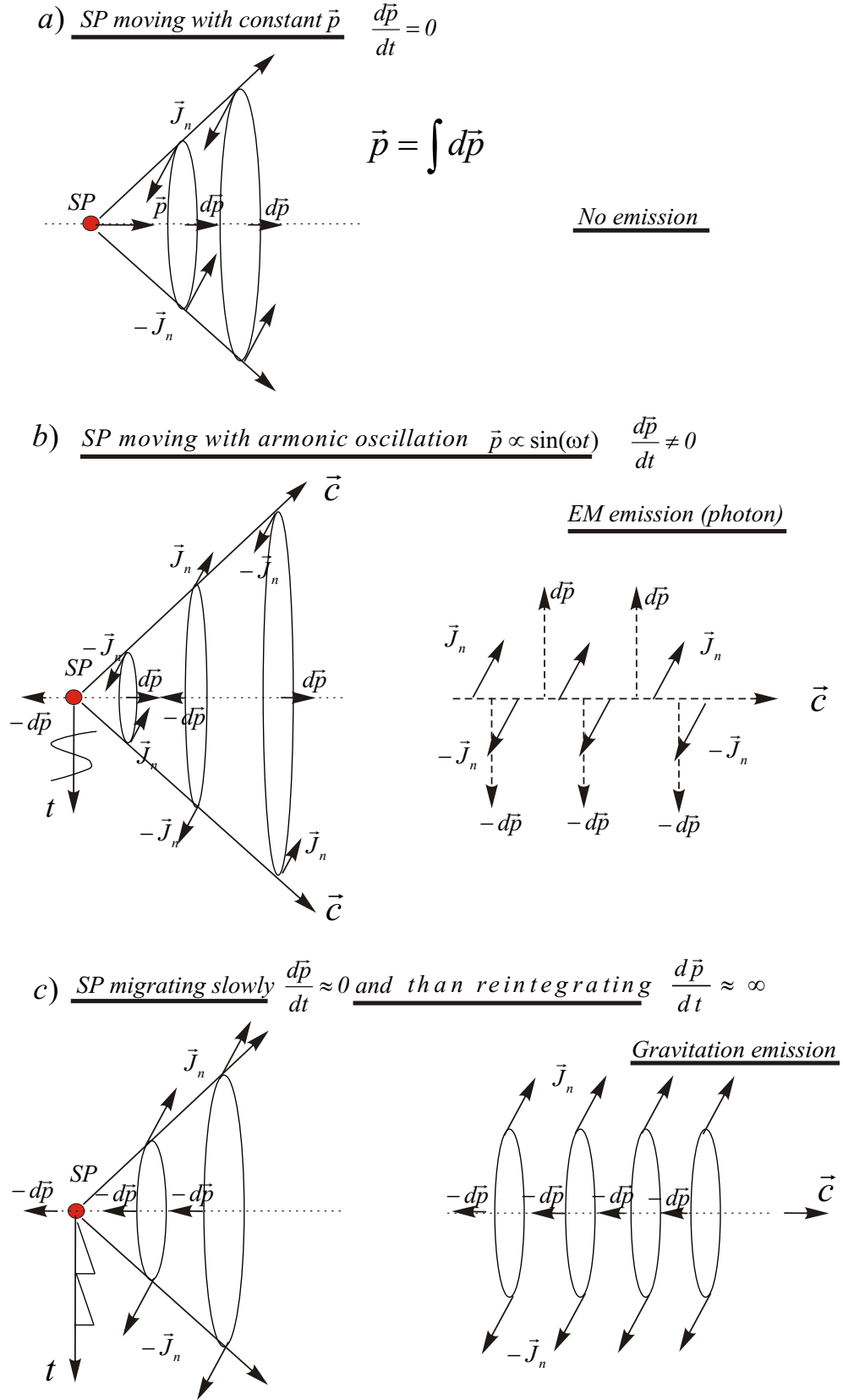
Figure 20: Electromagnetic and Gravitation emissions
