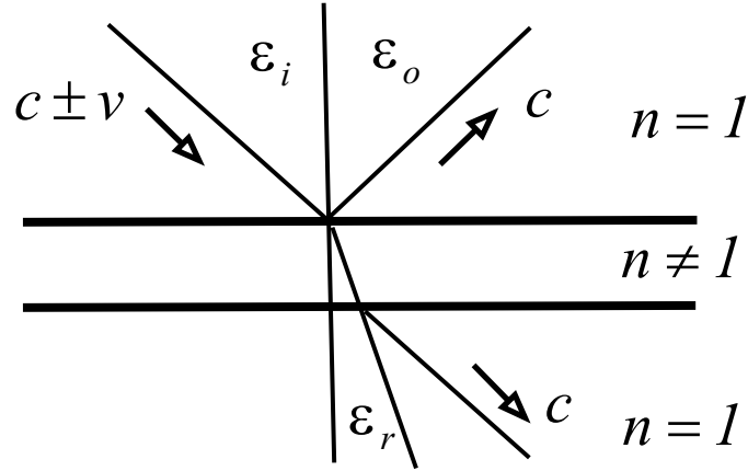
Figure 27: Light speed at reflections and refractions
