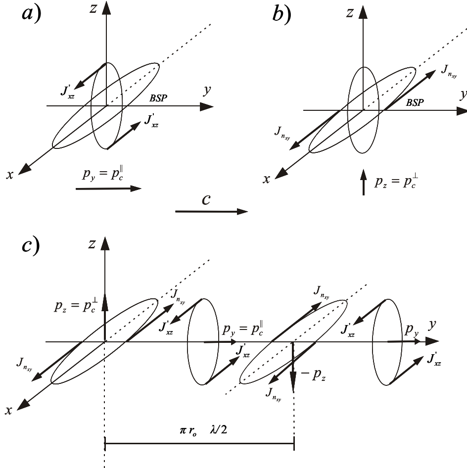
Figure 32: Different forms of BSP with light speed
