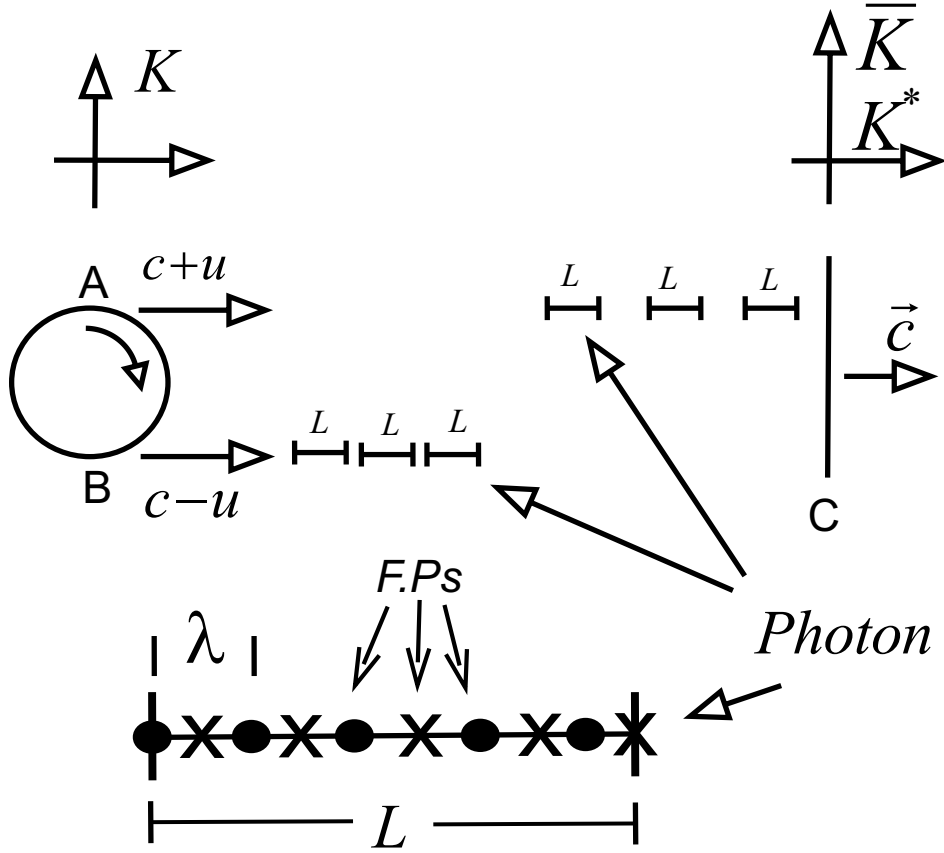
Figure 26: Emission Theory.
