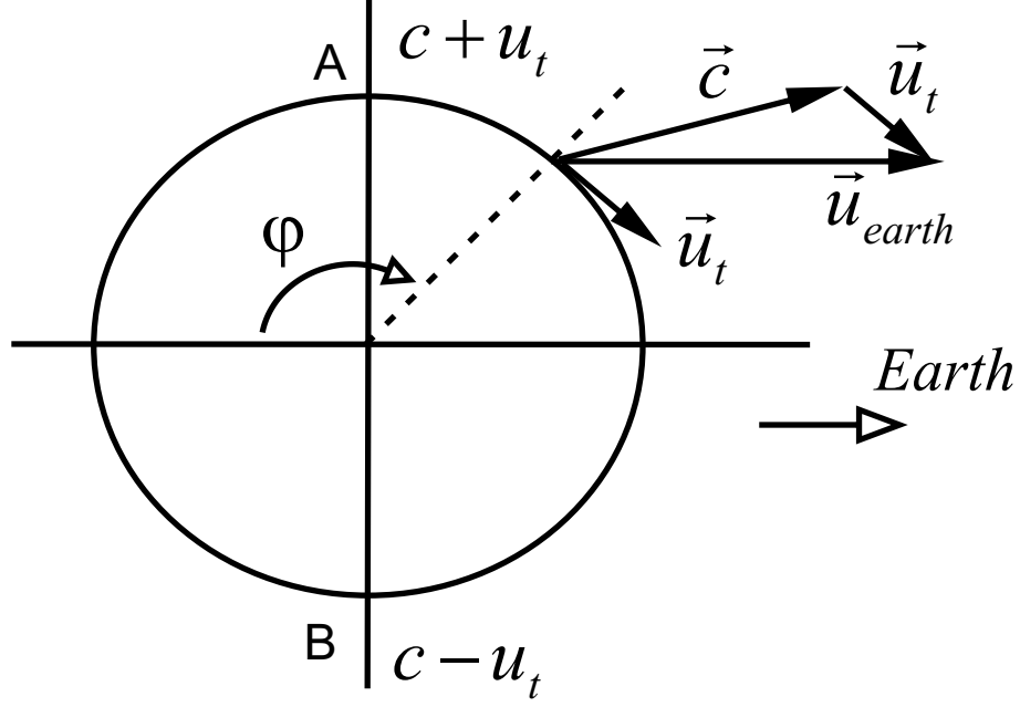
Figure 29: Speed of photons at an Binary Pulsar.
