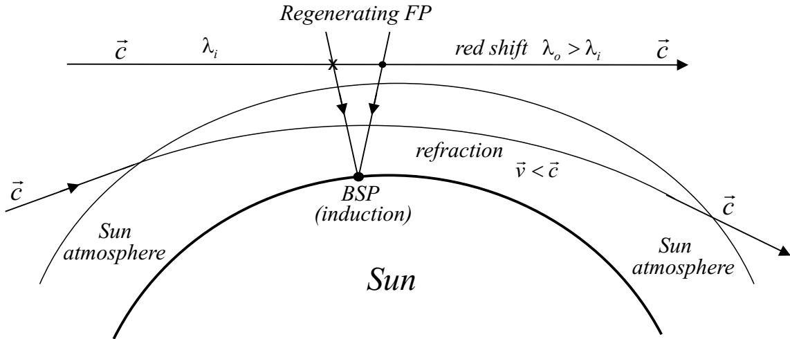
Figure 34: Refraction and red-shift at the Sun
