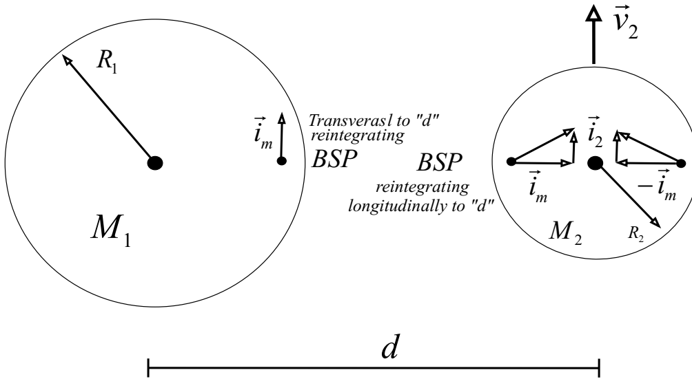
Figure 16: Ampere gravitation
