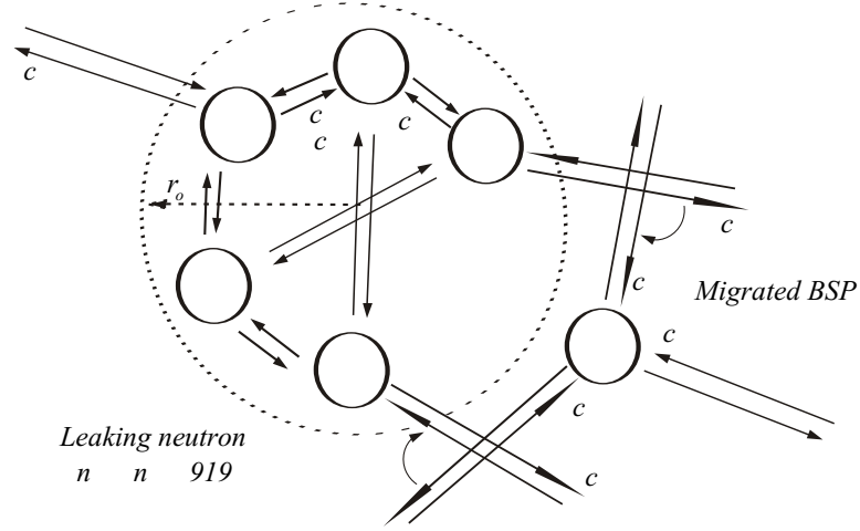
Figure 23: Neutron with migrated BSP
