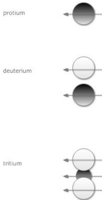
Hydrogen isotopes
